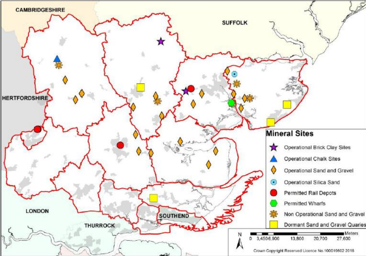
Figure 1: Mineral Extraction and Transshipment Sites (31 Dec 2017)
